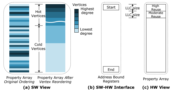
Figure 1: GRASP overview.
